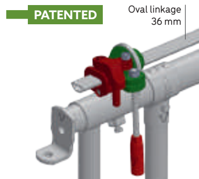
Folding control single-handed handle
