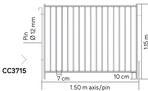
CC3715 Vertical goat hurdle H. 1.15 m L. 1.50 m vertical with pin - Available in packs of 12
