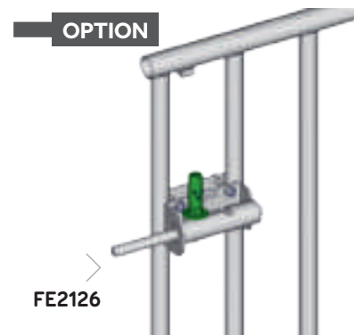
Adaptable AUTOLOCK bolt
