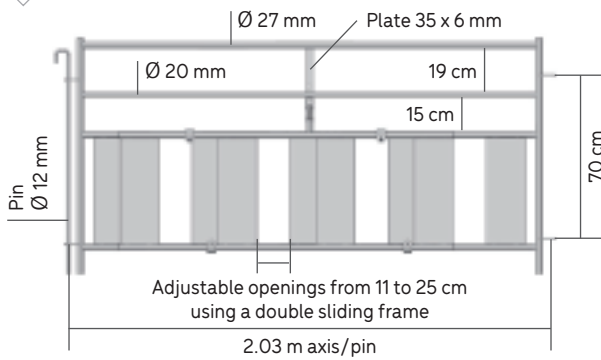
OV3705 Sheep hurdle 7 bars H. 1 m L. 2 m lamb creep with pin Available in packs of 6
