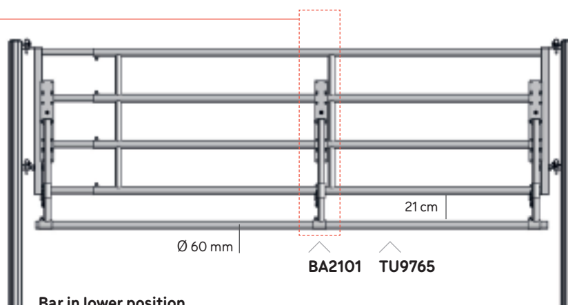
Bar in lower position
