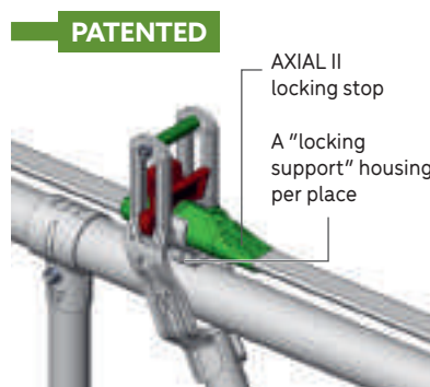
Individual central locking
