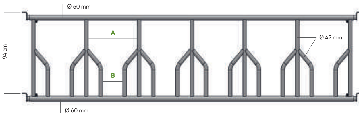
LS feston installation
