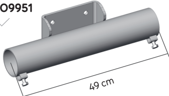
HEA front screen support
